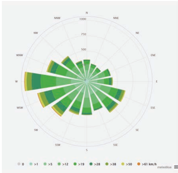
WIND ROSE OF LIVI
